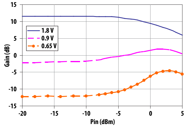
Figure 10. Gain vs. Pin at 6 GHz
