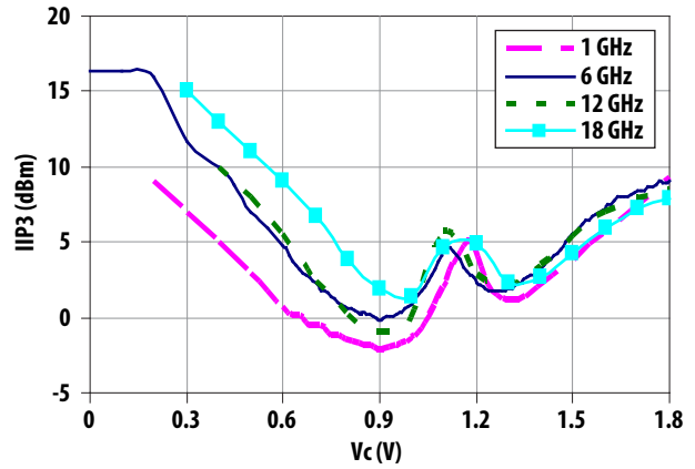
Figure 8. Input IP3 vs. Vc
