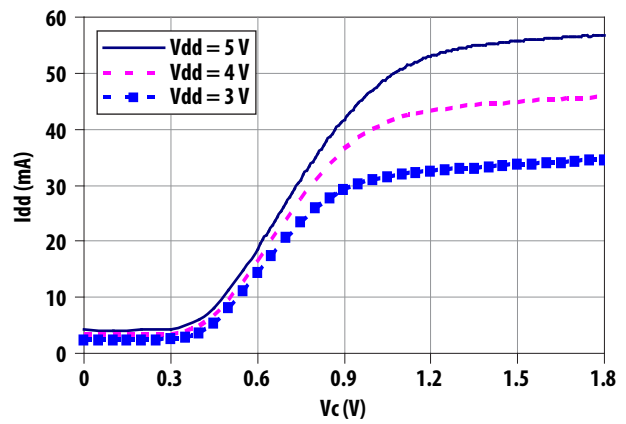
Figure 12. Supply Current over Bias
